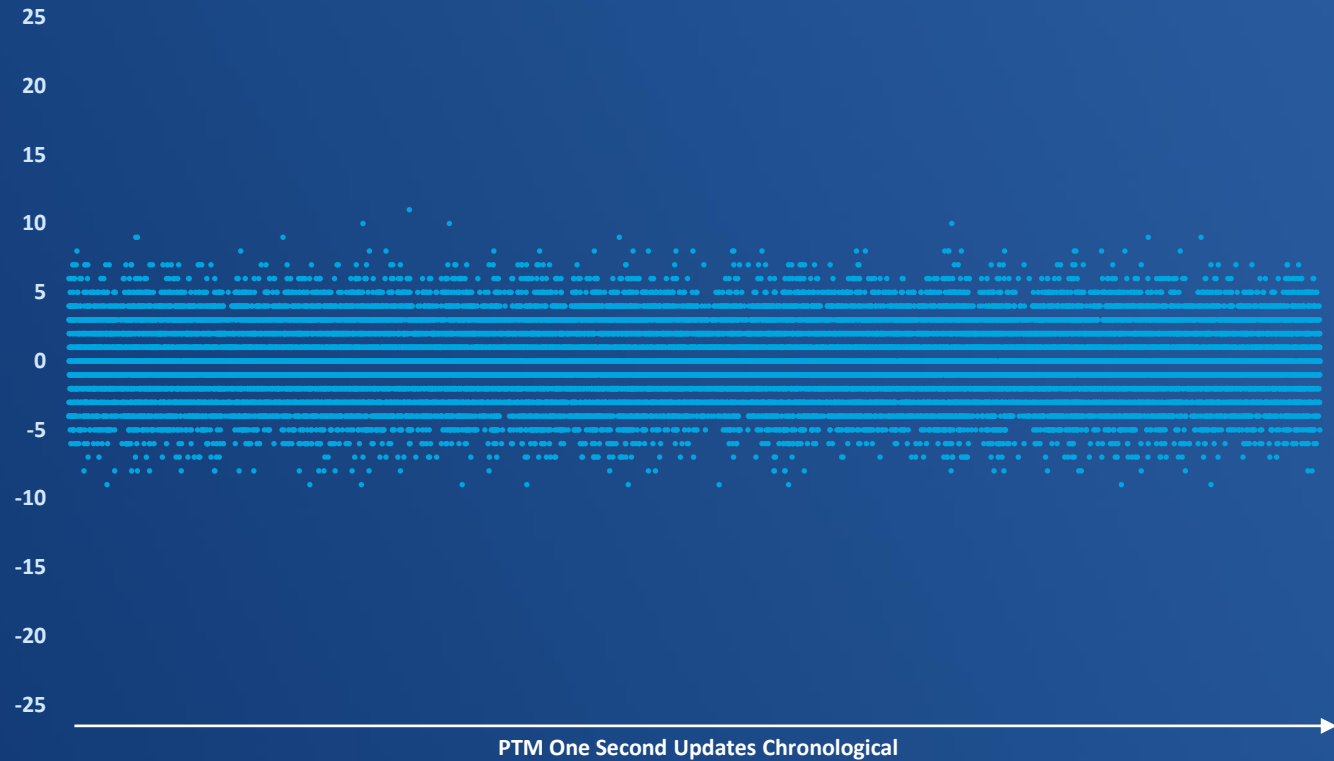
Host/ÜberNIC Host Real-Time Clock Post-Update Time Value Divergence
