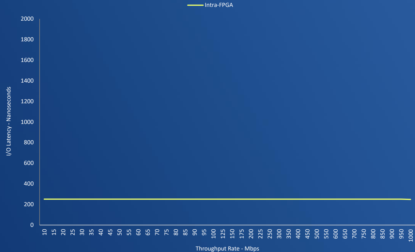
SOF FIFO Transceiver-to-Transceiver I/O Latency
